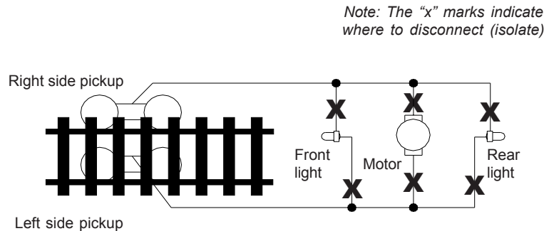
Figure 1. Connection of standard locomotive
