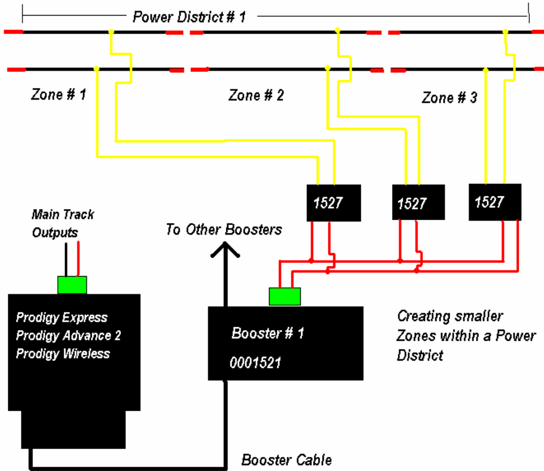
Figure # 2- Creating smaller zones within your power district using boosters.
