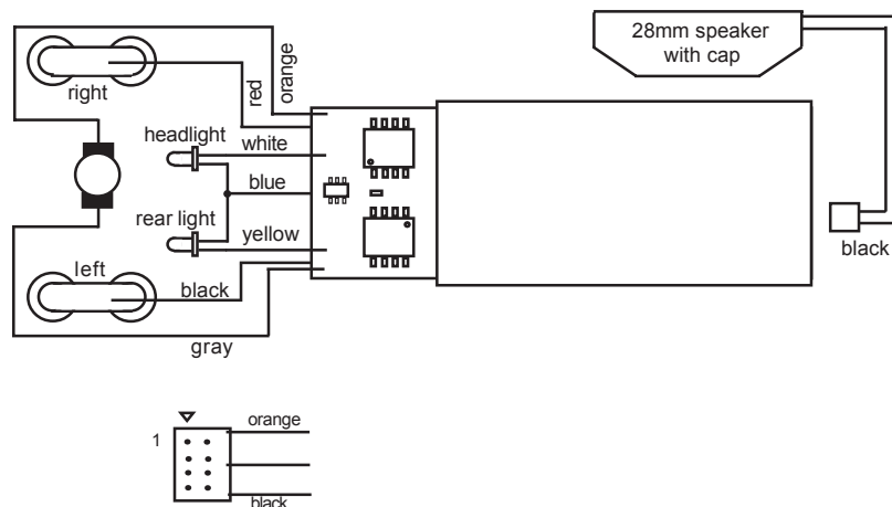
Figure 2. 0001629 decoder wiring diagram
