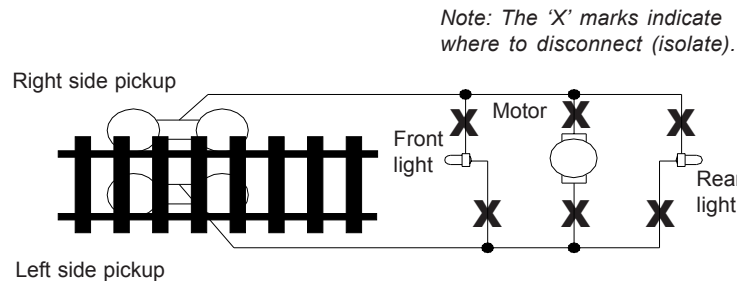
Figure 1. Connection of standard locomotive
