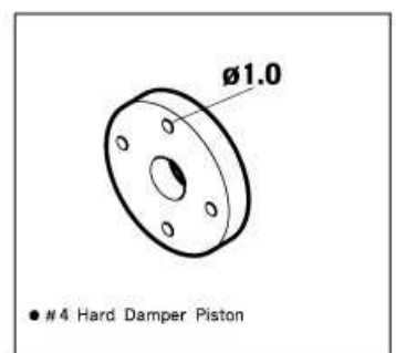
ST-T89 #4 Hard Damper Piston
