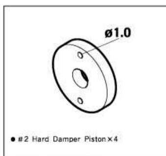
ST-T87 #2 Hard Damper Piston
